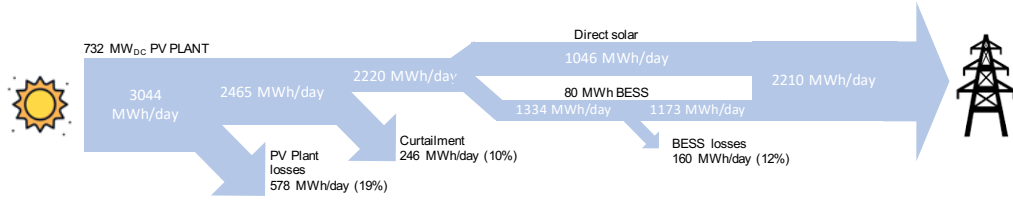
Figure 9: Sankey diagram of the project (average day).
